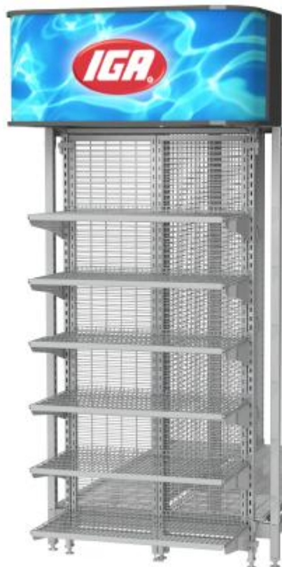
POSITION No. 2 FOLDED IN WITH WIRE SHELVES
